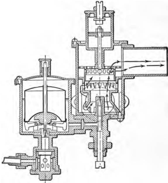
FIG. 160.—The Pierce Automatic Float-feed Sprayer, with arrows showing course of air through the mixing chamber to cylinder.
